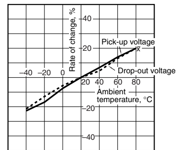
9. Ambient temperature characteristics Tested sample: TQ2SA-12V, 5 pcs.
